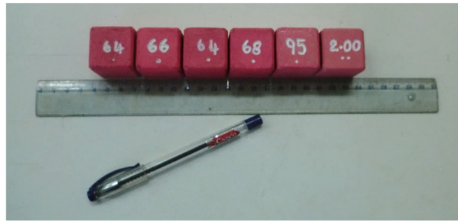
Figure 3. Cubic density tracers.
