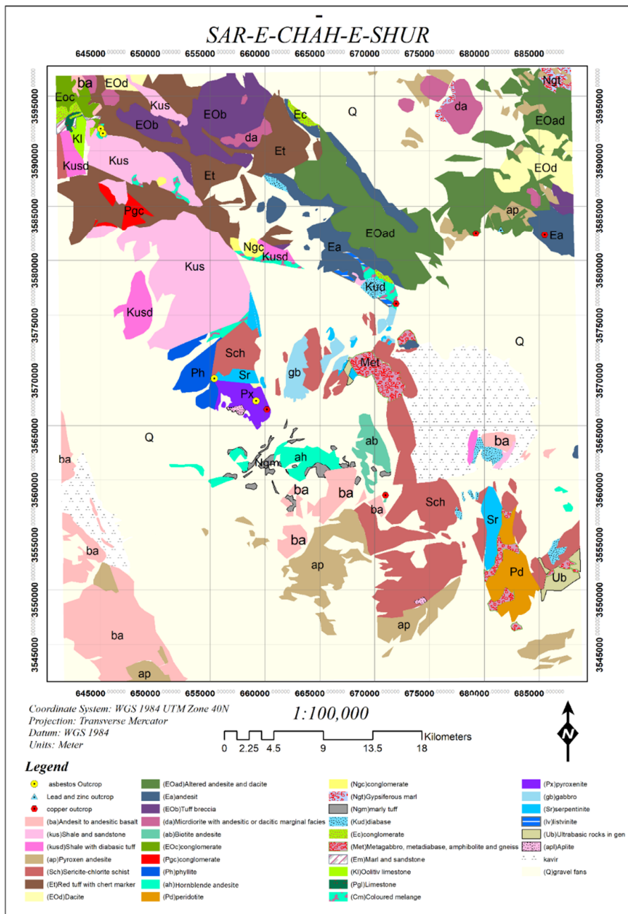
Figure 1. The 1:100,000 simplified geological map of the sar-châh-e-Shur well area.
