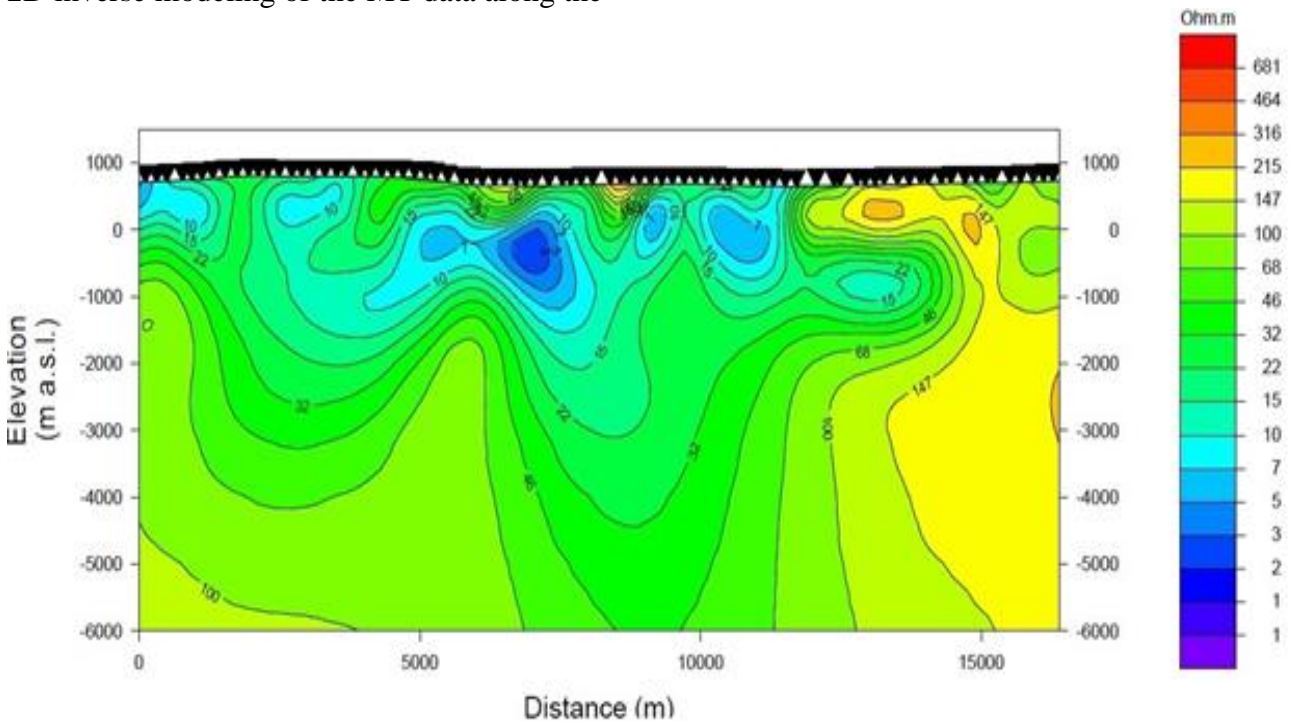
Figure 5. 2D-modeling along survey line 8807.
