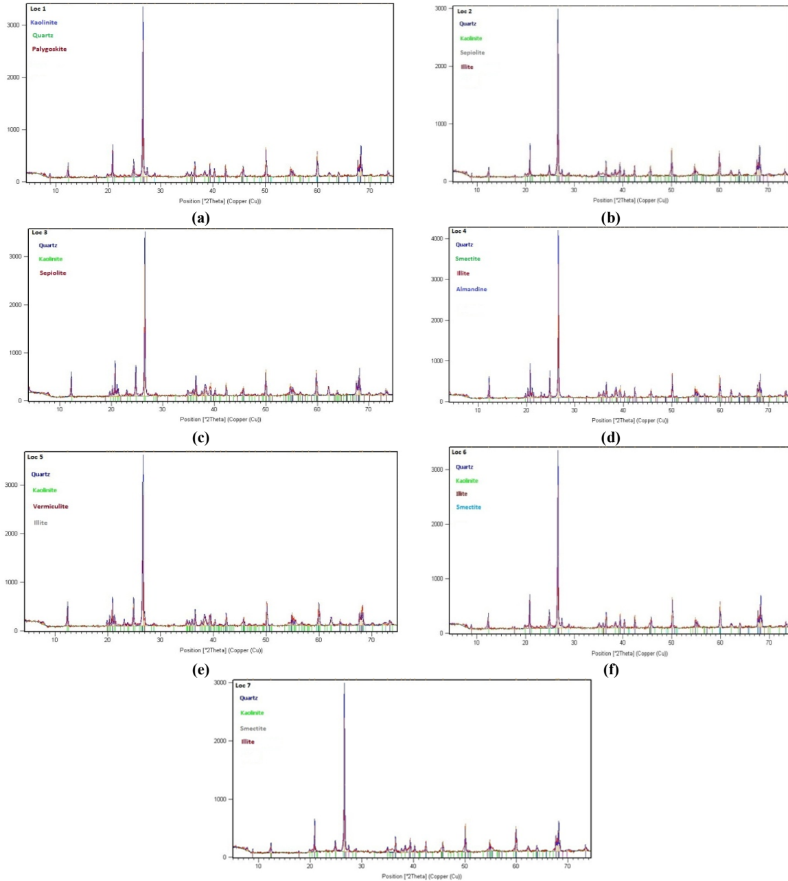
Figure 8. X-ray patterns of clay mineral in sample Loc 1 (a), Loc 2 (b), Loc 3 (c), Loc 4 (d), Loc 5 (e), Loc 6 (f), Loc 7 (g)
