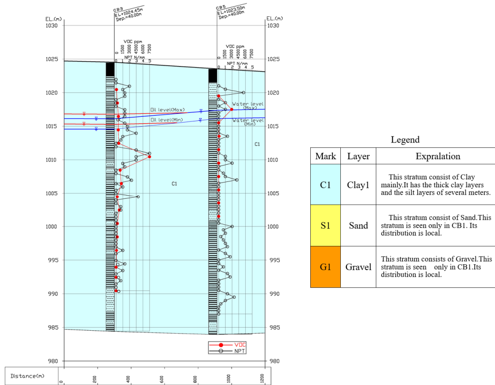
Figure 4. Geological profile of CB3~CB5 [78].
