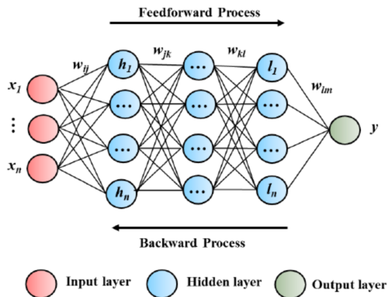
Figure 1. Schematic of an MLP neural network structure [39].
