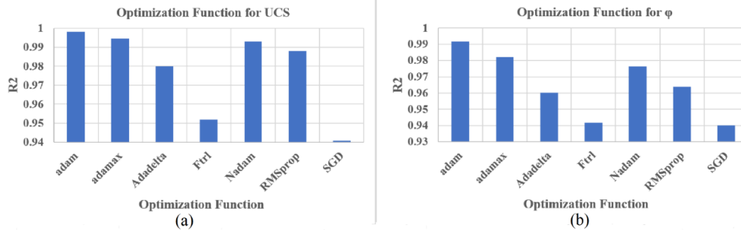
Figure 5. A comparison of the R² (coefficient of determination) values obtained for UCS (a) and φ angle (b) predictions with various optimizer functions using the CL algorithm for blind data.
