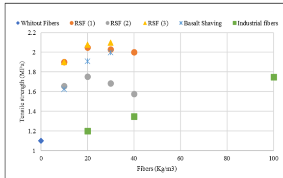
Figure 9. Tensile strength diagram of samples without fibers, with fibers and, containing basalt shavings.
