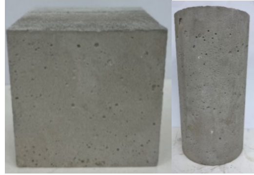
Figure 4. Cubic (10×10×10 cm) and cylindrical (15×30 cm) samples
