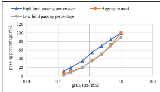
Figure 1. Granulation diagram of the used sand
