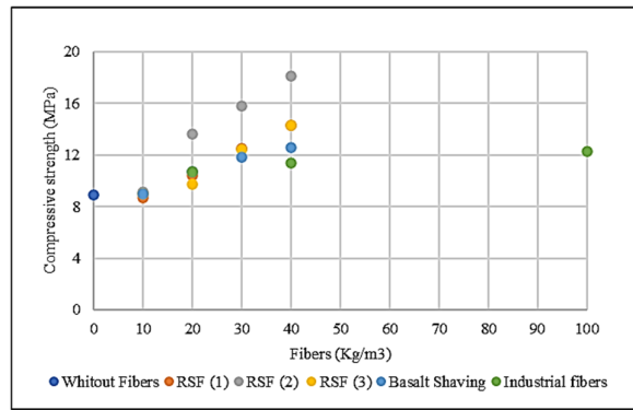
Figure 6. Compressive strength diagram of samples without fibers, with fibers, and containing basalt shavings.
