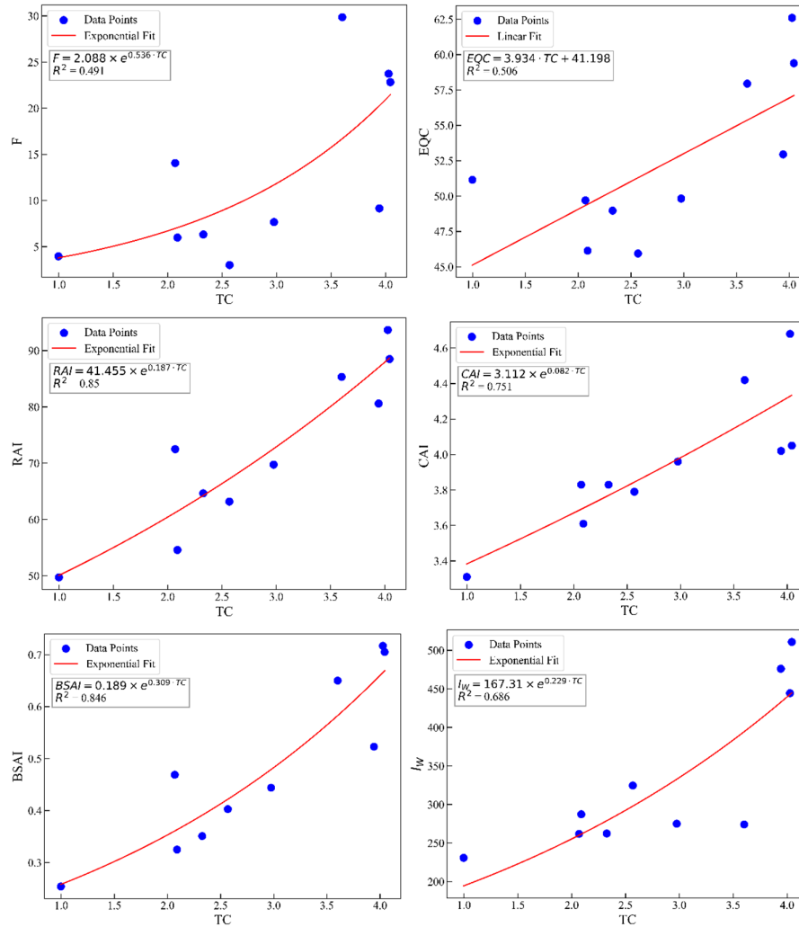
Figure 2. Relationships between TC and abrasivity indices.
