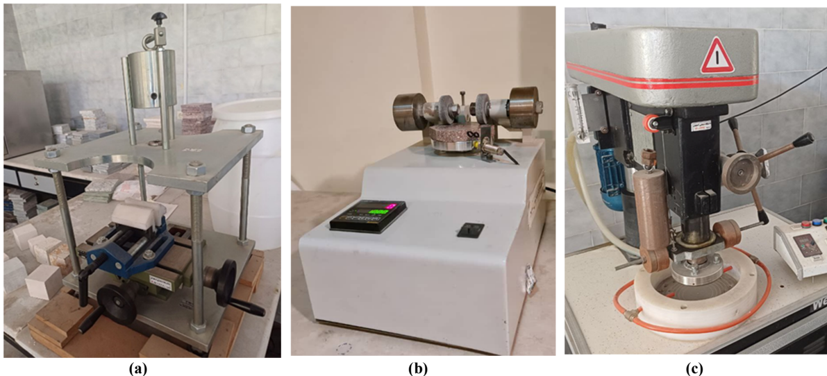
Figure 1. Equipment for measuring abrasivity properties of studied stones: a) West Cerchar abrasivity index tester, b) Taber Abraser tester 5130, and c) BSAI laboratory test rig.
