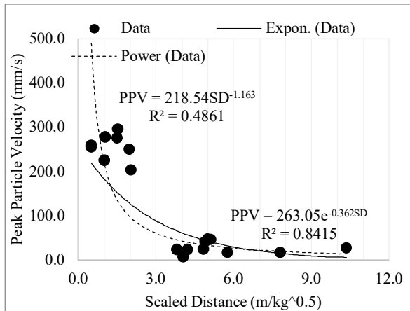
Figure 5. Mathematical equation for wave attenuation of the signature blast holes in Golgohar Mine
