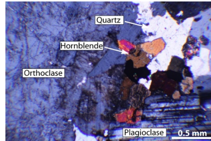
Continuous of Figure 3. Microscopic characteristics of the studied rock samples.
