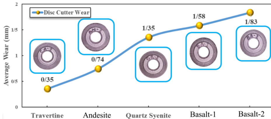
Figure 7. Average wear of cutting disc of the small-scale linear cutting machine in different rock samples.
