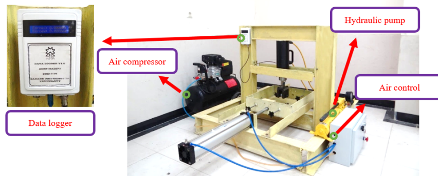
Figure 5. The full view of the small-scale linear cutting machine in the mechanized excavation laboratory of Sahand University of Technology.
