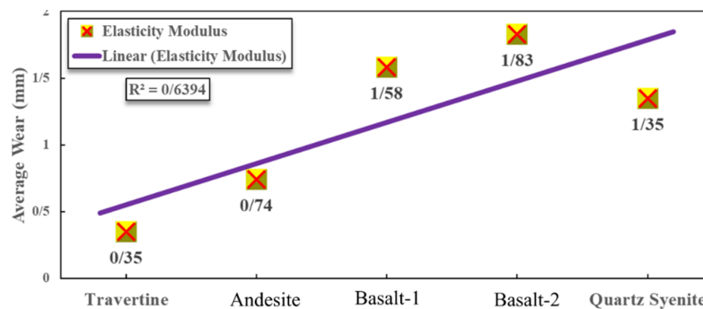
Figure 11. Changes in the wear of the disc cutter according to the values of the modulus of elasticity in 5 different rock samples.
