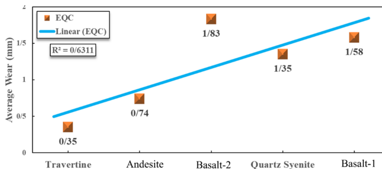
Figure 10. Changes in disc cutter wear regarding equivalent quartz content (EQC) in 5 different rock samples.
