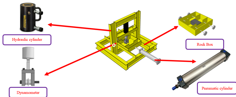
Figure 4. 3D schematic of the designed small-scale linear cutting material.
