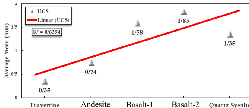
Figure 8. Changes in disc cutter wear according to the uniaxial compressive strength of rocks in 5 different rock samples.
