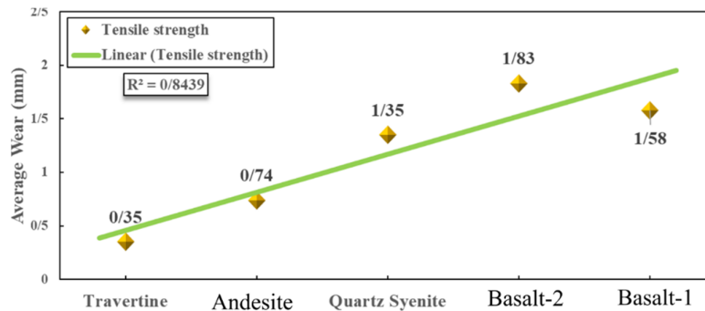
Figure 9. Changes in disc cutter wear according to Brazilian tensile strength in 5 different rock samples.
