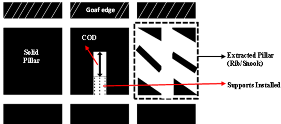
Figure 2. Schematic view of mechanized depillaring workings
