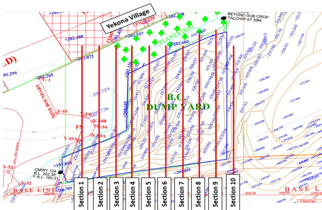
Figure 5. Cutting line over contour map for actual cross-sections
