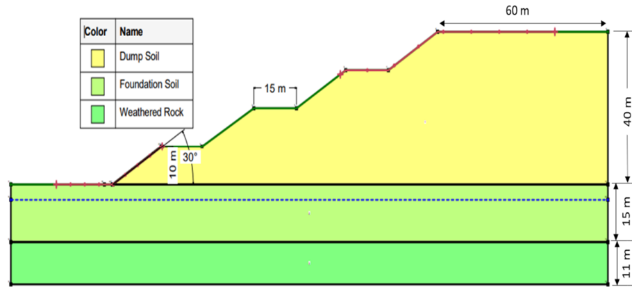
Figure 7. Recommended cross-sections to be followed at the site
