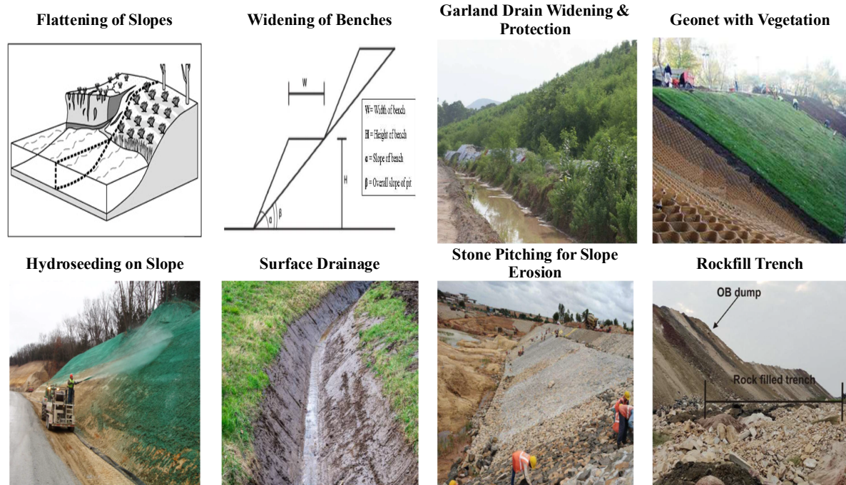
Figure 9. Remedial measures for the BC soil dump
