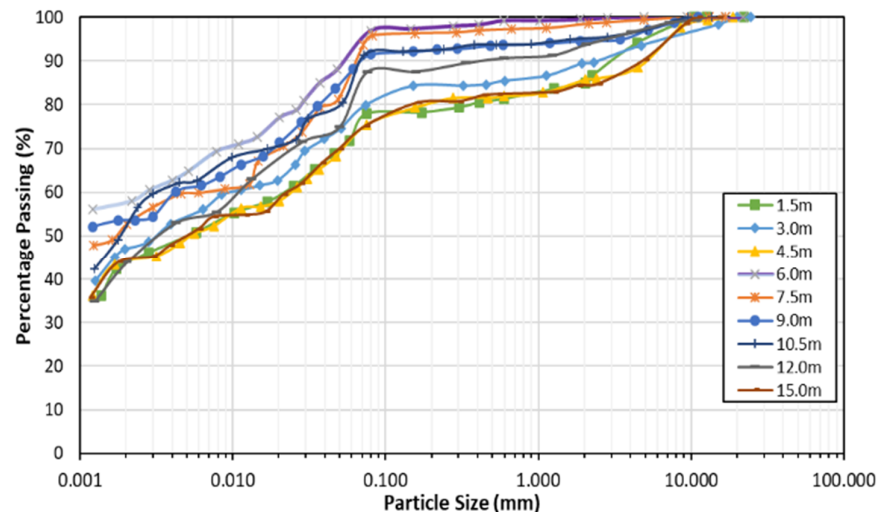
Figure 4. Grain size distribution curve for samples taken from different depths in the BH1 borehole
