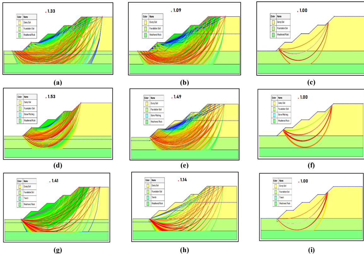
Figure 8. Analysis results for variation in FoS: (a), (b), and (c) for the effect of saturation; (d), (e), and (f) for effect of stone pitching; (g), (h), and (i) for the effect of rockfill trenching
