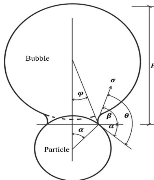
Figure2. Model of mineral particle attached air bubble
