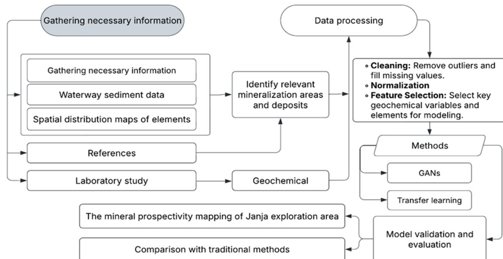
Figure 4. Research Methodology
