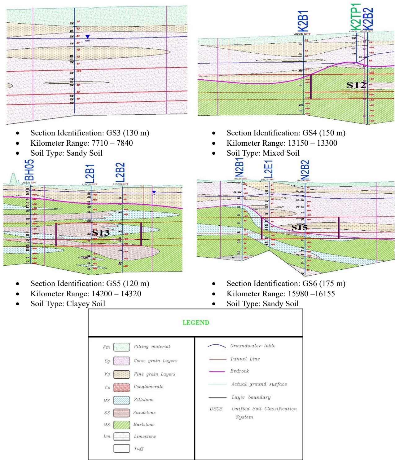
Continuation of Figure 7. Geotechnical Profile and Subsurface Information of Selected Sections (The depth of the profile is down to -30 meters).
