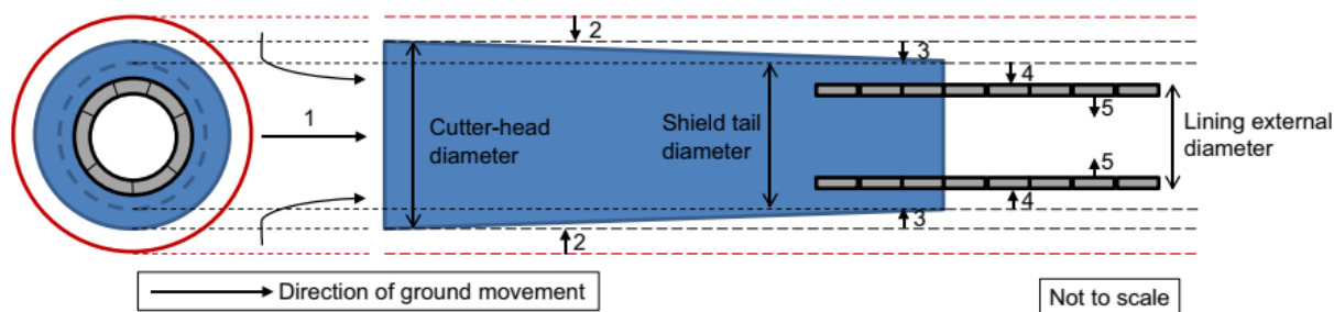
Figure 3. Illustration on components of volume loss [34].
