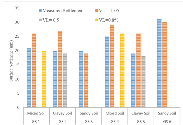
Figure 15. Comparative Settlement Graphs from Numerical Method at Various Volume Loss (VL) Values
