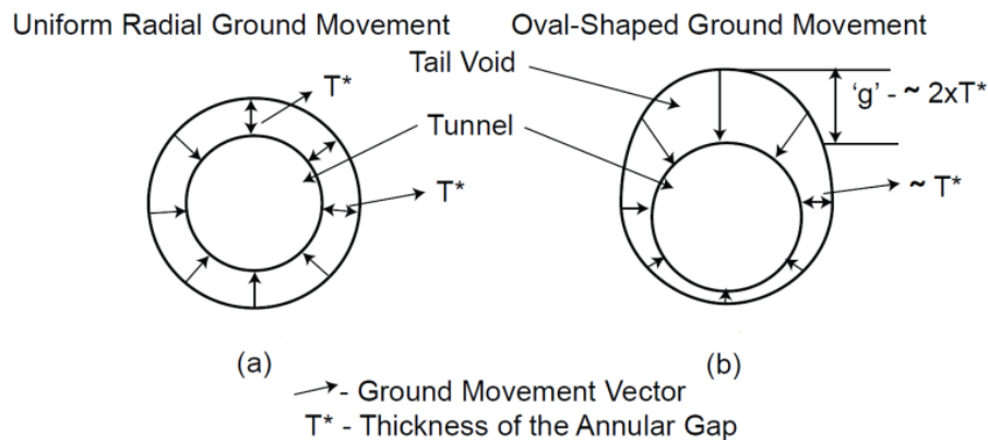
Figure 2. Circular and Elliptical Deformation Patterns Around Tunnels [32].
