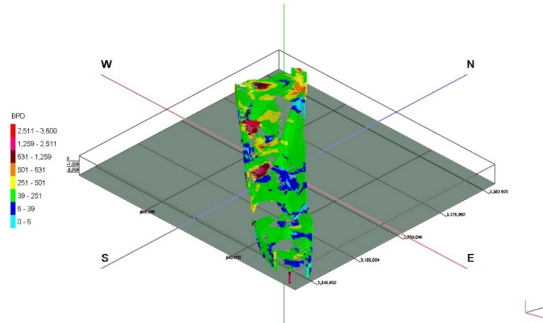
Figure 8. Permeability zones' distribution map of the permeability via the C-V model in the Gachsaran oilfield.
