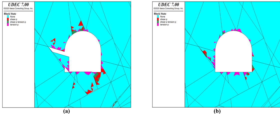
Figure 6. Plastic zone around the models for P_{32} = 1.0\text{m}^2/\text{m}^3 indicated by the Mohr Coulomb failures criterion for a) \varphi = 10^\circ and b) \varphi = 30^\circ
