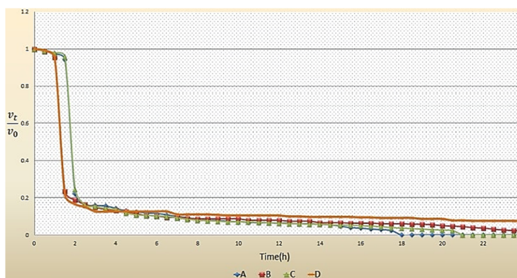
Figure 3. Voltage-time ratio graphs for batteries discharging in solutions containing salts A, B, C, D at a 20% mass concentration using a high-speed magnetic stirrer
