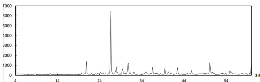
Figure 4. XRD of ore sample
