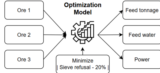
Figure 2. Optimization model linking ore inputs to process controls.
