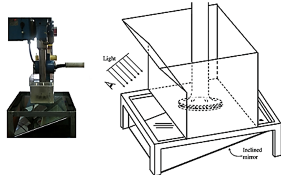
Figure 2. Experimental scheme used to measure the critical impeller speed.
