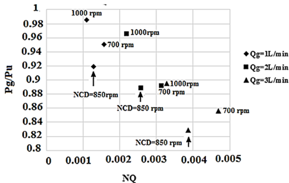
Figure 3. The relationship between N_q and P_g/P_u
