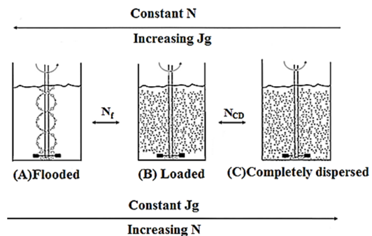
Figure 1. Schematic picture of the bulk flow patterns.
