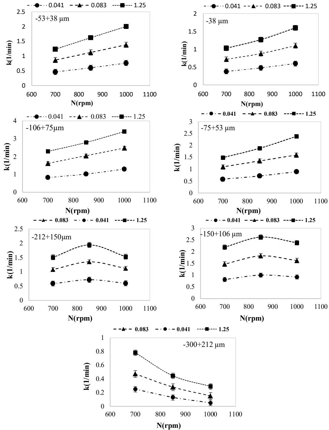
Figure 4. The relationship between impeller speed and flotation rate constant at different particle sizes and superficial gas velocities.
