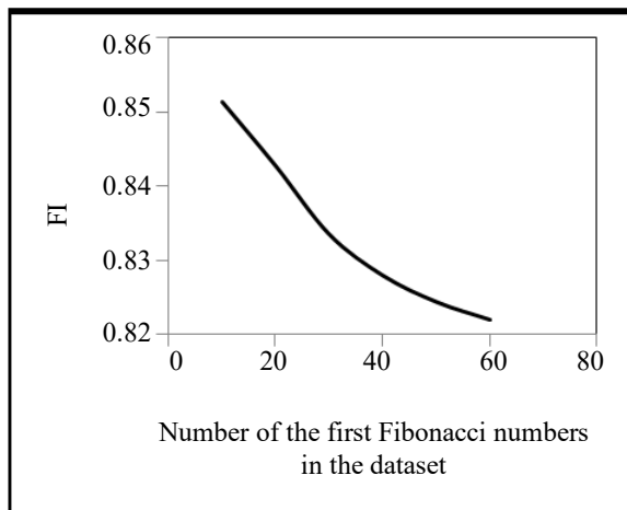
Figure 8. FI (division of standard deviation of Fibonacci Transformed data (Fibstdev) by raw data standard deviation) versus number of the first Fibonacci numbers
