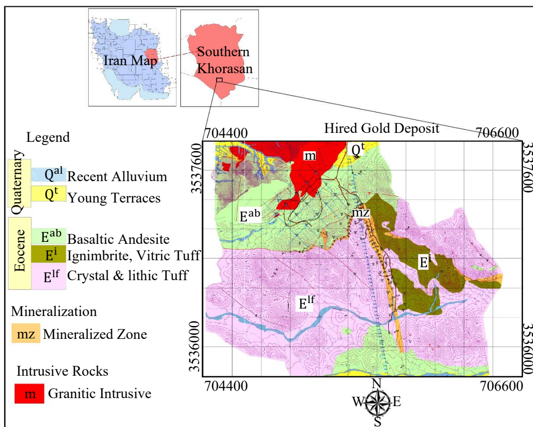
Figure 9. Simplified Hired gold deposit geological map
