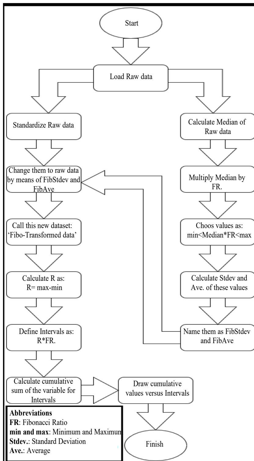
Figure 5. Flowchart of the Fibonacci Transformation method
