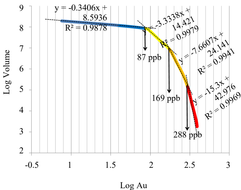
Figure 13. Concentration-Volume log-log plot
