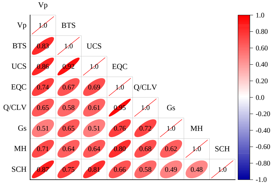
Figure 9. Pearson correlation between stone properties
