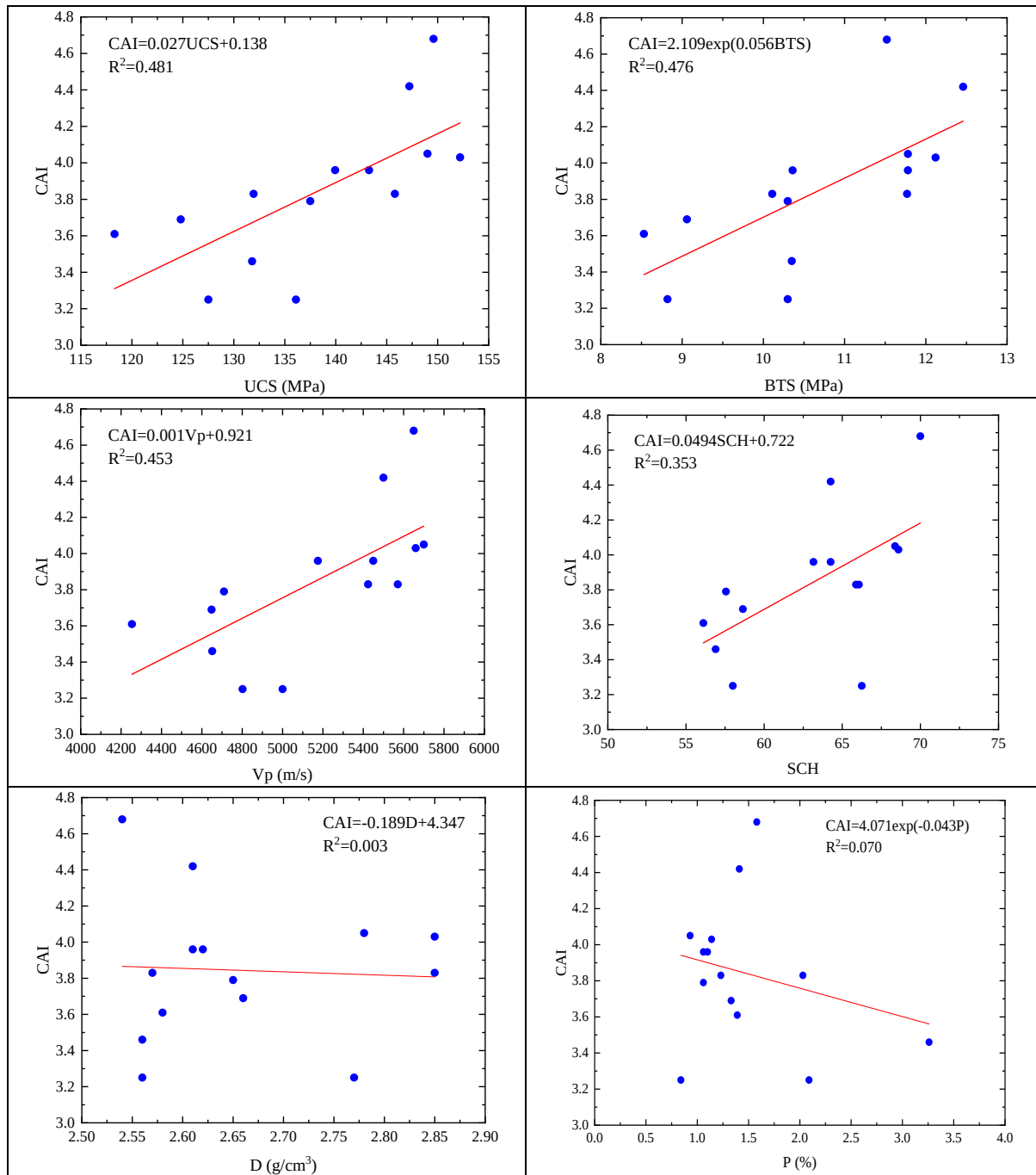
Figure 8. Relationship between CAI and physico-mechanical properties
