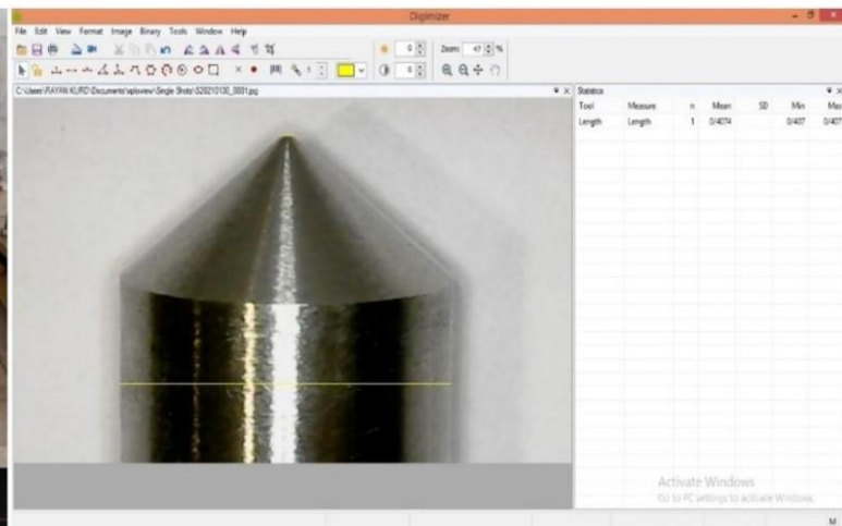
Figure 4. Measurement of wear flat on the steel stylus tip by (a) high-resolution camera, and (b) Digimizer software
