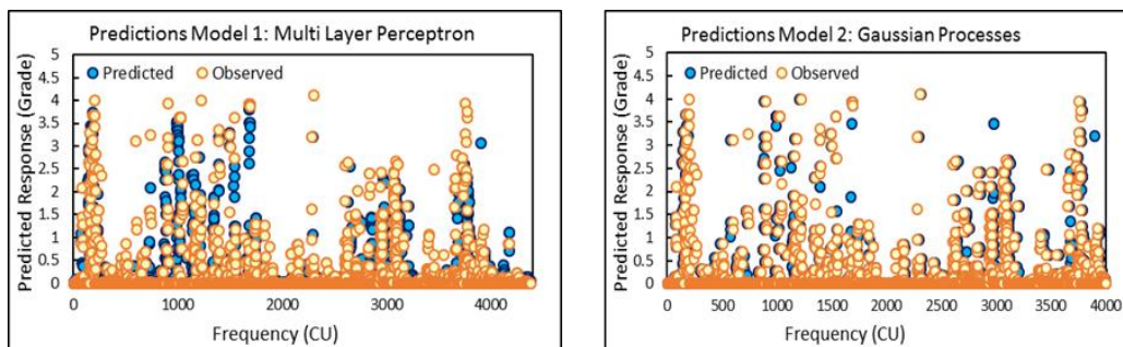
Figure 6. Qualitative evaluation results of network performance on training data for the methods used in copper grade estimation.
