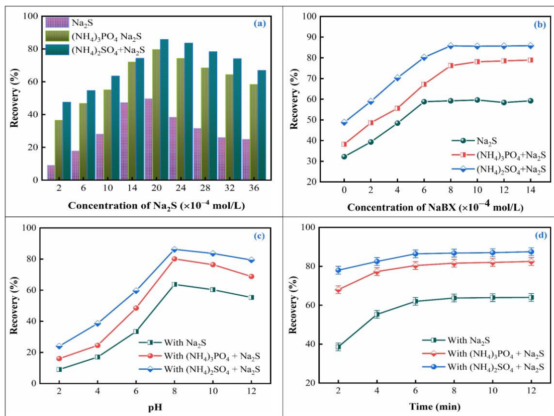
Figure 2. Micro-flotation recovery of malachite as a function of (a) Na 2 S, (b) NaBX concentrations, (c) pH, and (d) time conditions.
