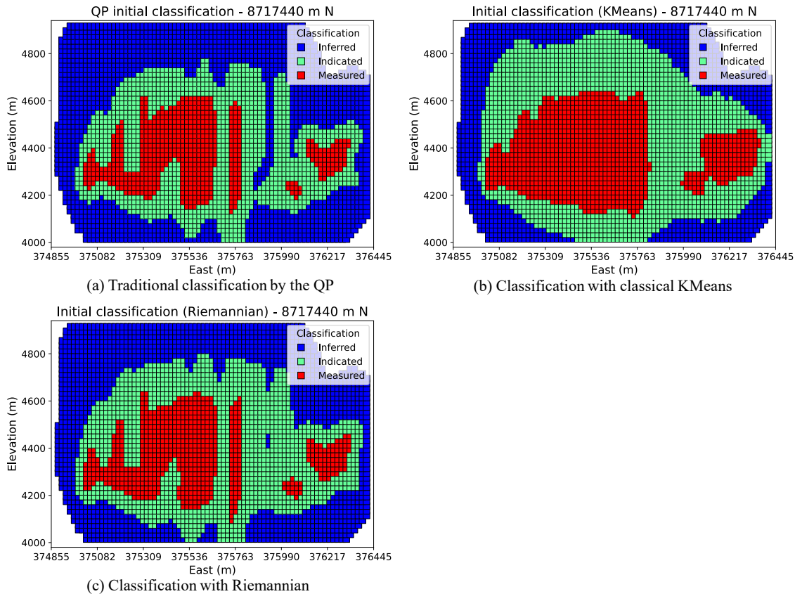
Figure 6. Block classification comparison at section 8717440 m N
