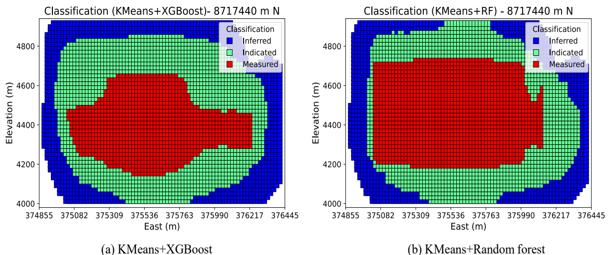
Figure 8. Classification smoothing of KMeans
