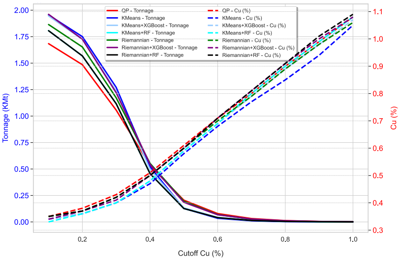
Figure 14. Tonnage vs. copper grade curves for the inferred resource class across models
