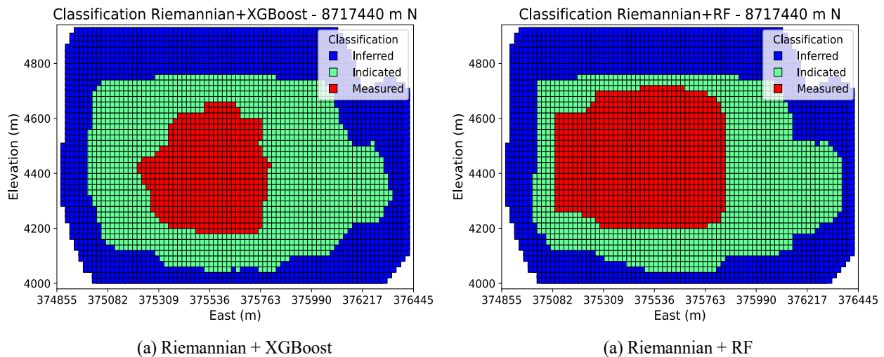
Figure 10. Classification smoothing of Riemannian
