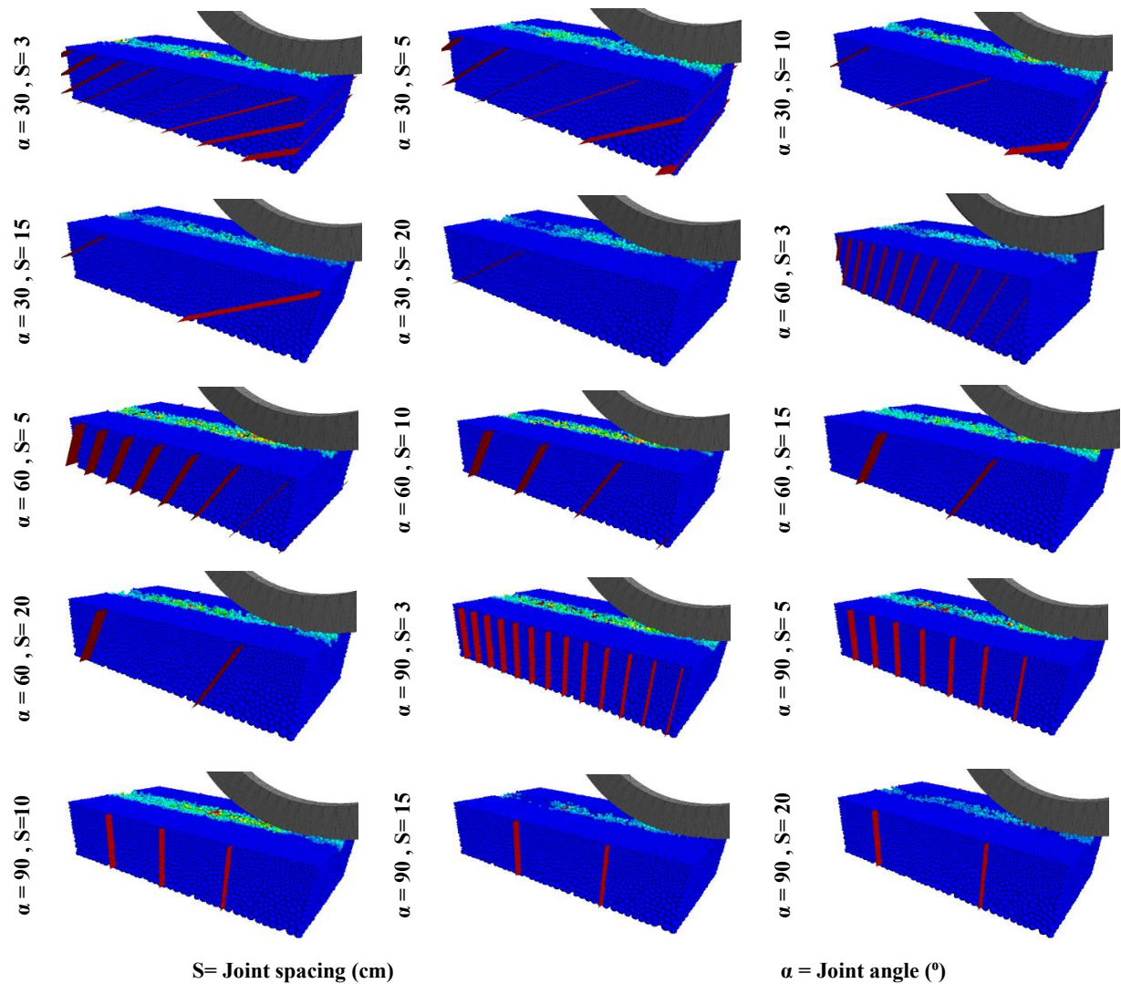
Figure 11. Applied joint in intact rock block with different spacing and angle
