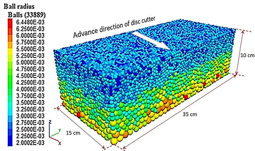
Figure 3. Simulated intact rock block
