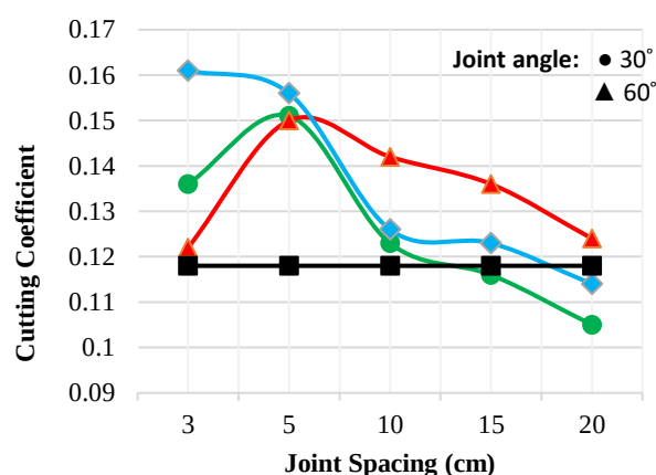
Figure 15. Correlation of the cutting coefficient with different joint spacing and dip angle
