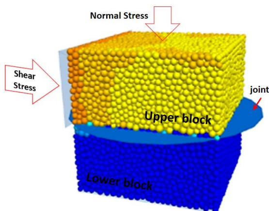
Figure 4. A view of direct shear test modeling
