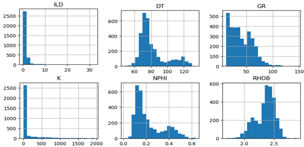
Figure 3. Histograms displaying the statistical distributions of the petrophysical variables: Gamma Ray (GR), Neutron Porosity (NPHI), Bulk Density (RHOB), Sonic (DT), induction resistivity (ILD) and Core Permeability (K).
