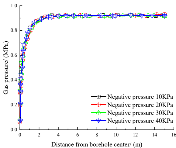
Figure16. Gas pressure distribution around the borehole under different negative drainage pressures
