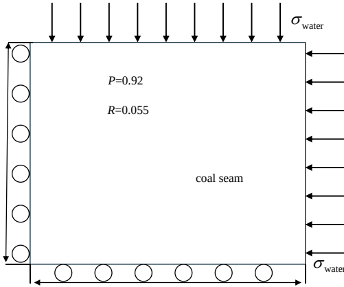
Figure 10. Computational geometric model and boundary conditions
