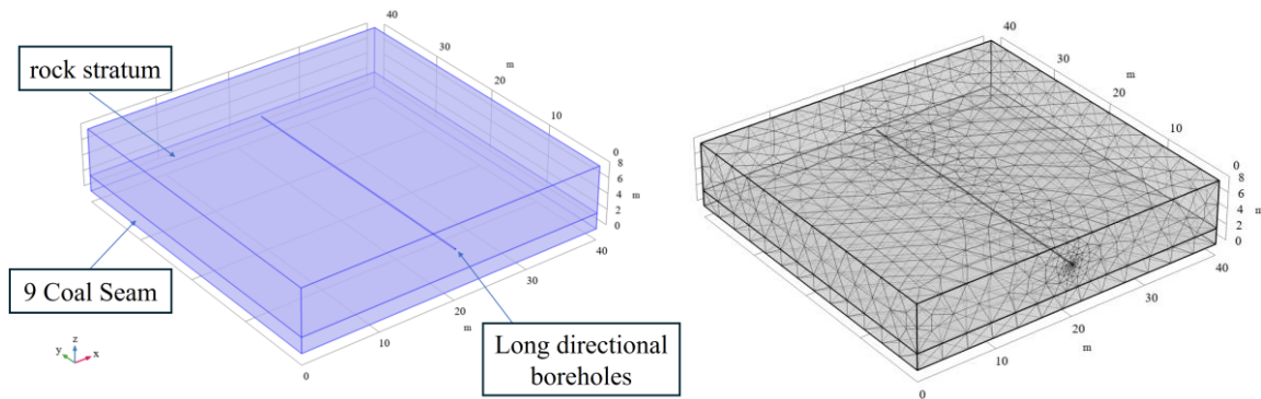
Figure2. Borehole model after grid delineation
