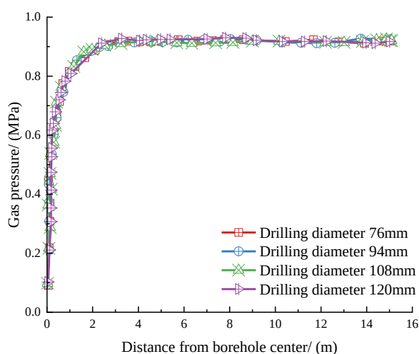
Figure 14. Distribution of gas pressure around the borehole for different borehole diameters
