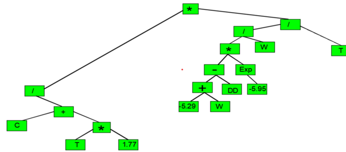
Figure 5. Final Expression Tree generated by GP
