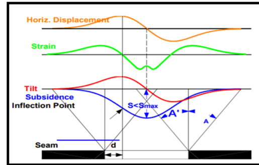
Figure 1. Factor schematic diagram of angle of draw
