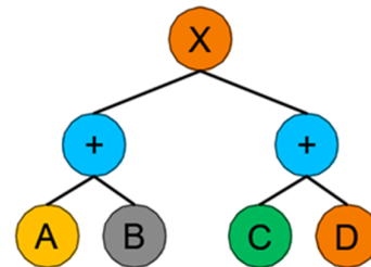
Figure 3. GP tree structure of (A+B) \times (C+D)
