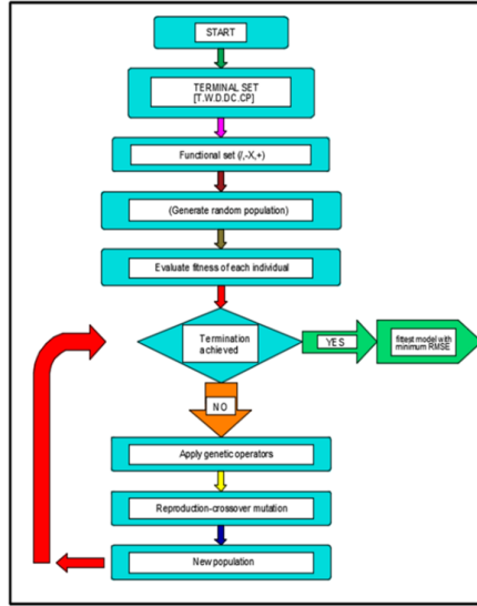
Figure 4. Sample flowchart of GP
