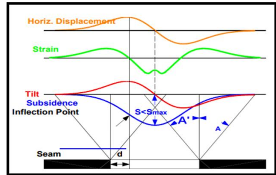
Figure 1. Factor schematic diagram of angle of draw
