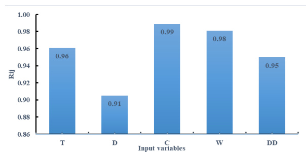
Figure 6. Results of SA obtained applying Cosine amplitude method
