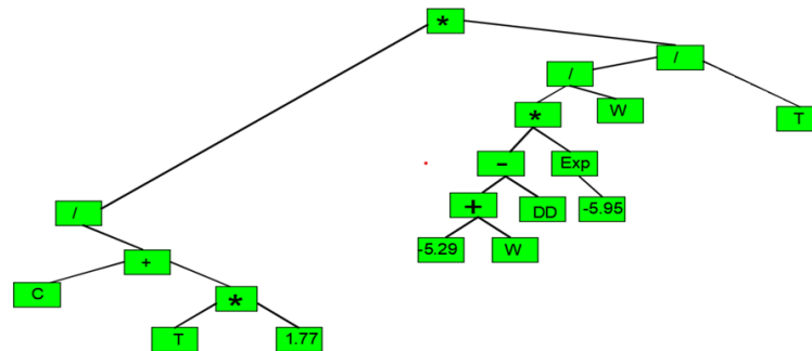
Figure 5. Final Expression Tree generated by GP
