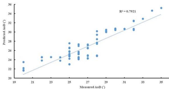
Figure 7. Actual vs predicted CP using GP on training dataset
