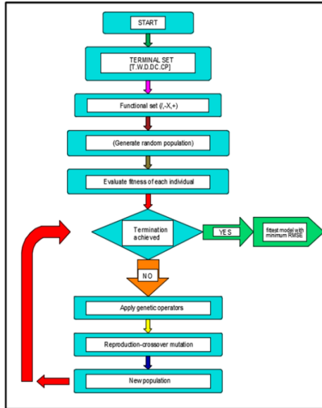
Figure 4. Sample flowchart of GP
