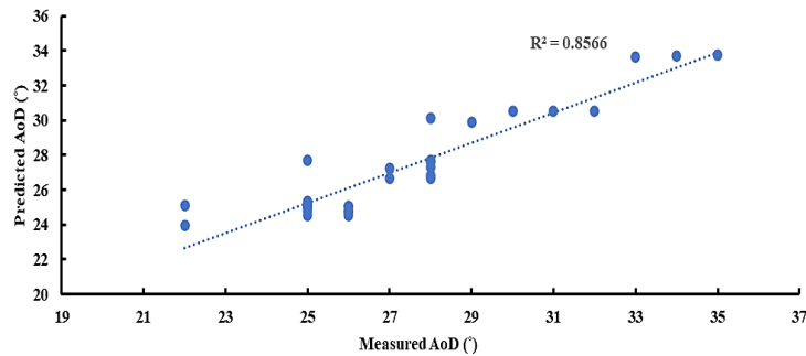
Figure 8. Actual vs predicted CP using GP on testing dataset
