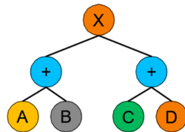
Figure 3. GP tree structure of (A+B) \times (C+D)
