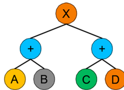
Figure 3. GP tree structure of (A+B) \times (C+D)
