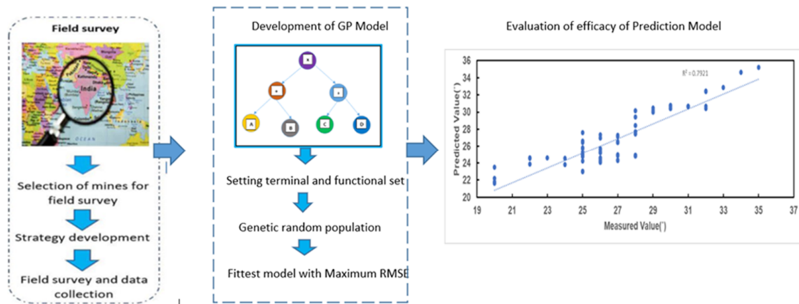
Figure 2. Methodology of the study
