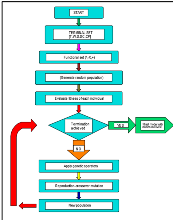
Figure 4. Sample flowchart of GP
