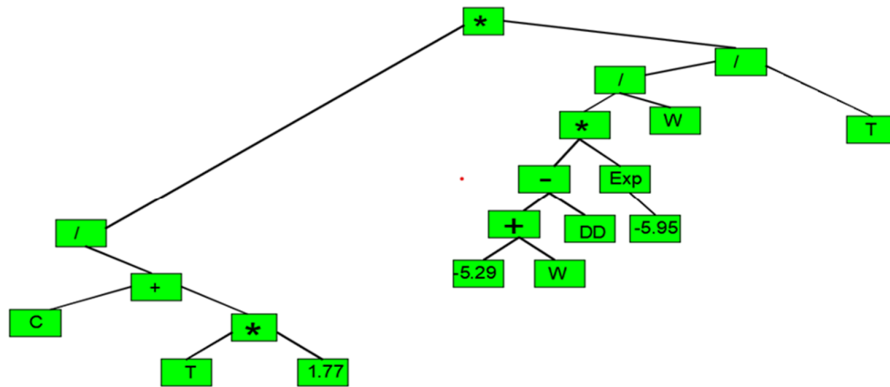
Figure 5. Final Expression Tree generated by GP
