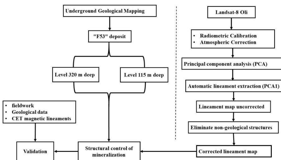
Figure 3. Methodology adopted for the study
