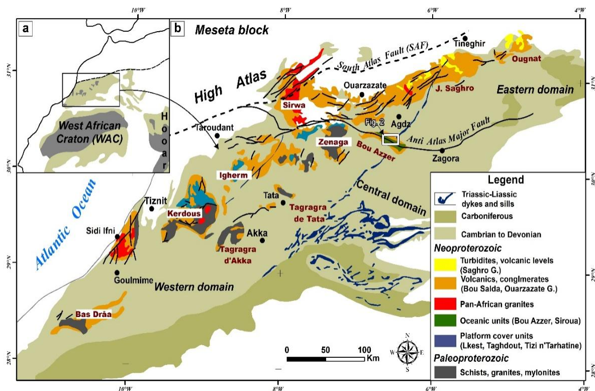
Figure 1. (a) The location of Moroccan anti – Atlas, (b) The general geological map of the anti-Atlas shows the location of the study area [26]
