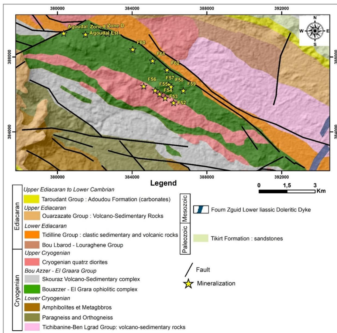
Figure 2. Geological map of the study area [15]
