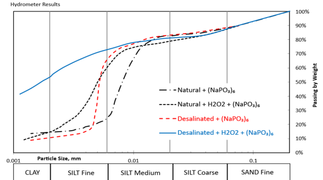
Figure 10. Hydrometer test results using Stokes' solution
