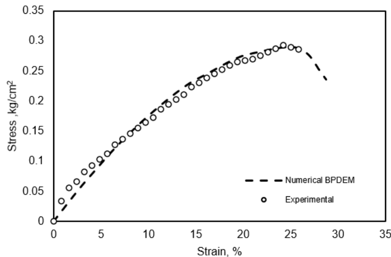
Figure 34. Comparison of force-displacement curves from numerical modeling and laboratory results for soft sediment under uniaxial compressive loading.
