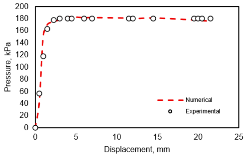
Figure 31. Comparison of numerical and experimental results from extrusion tests on remolded sediment samples with 45% moisture content.
