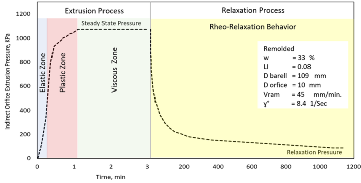
Figure 21. Pressure-time curve of the extrusion and relaxation process for remolded sediment with 33% moisture content.
