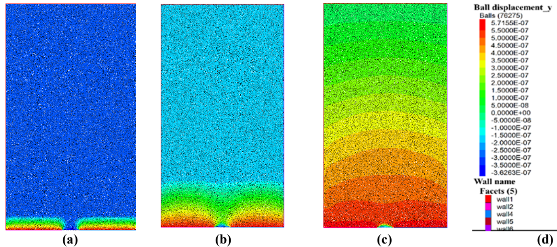
Figure 29. Displacement contour of the numerical extrusion test model during different loading and sediment discharge stages.
