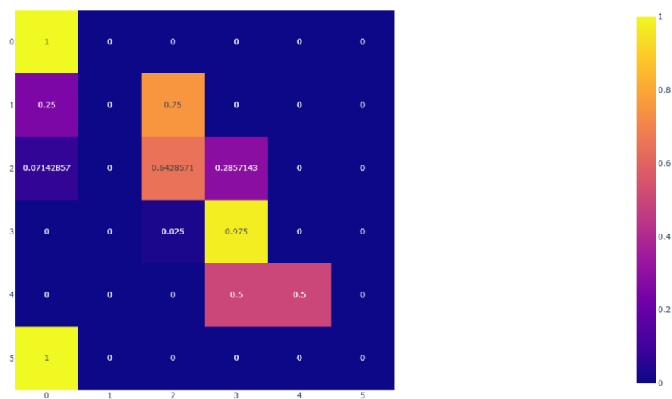
Figure 9. Confusion Matrix for Stability ClassesFigure
