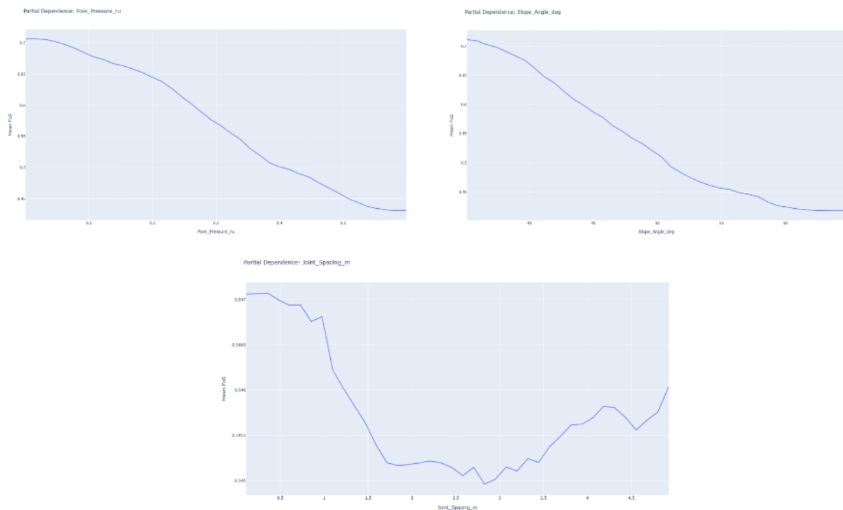
Figure 15. Partial dependency plot for all three regression
