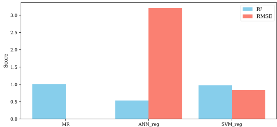
Figure 6. Comparison of Regression Accuracy Between MR, ANN, and SVM Models
