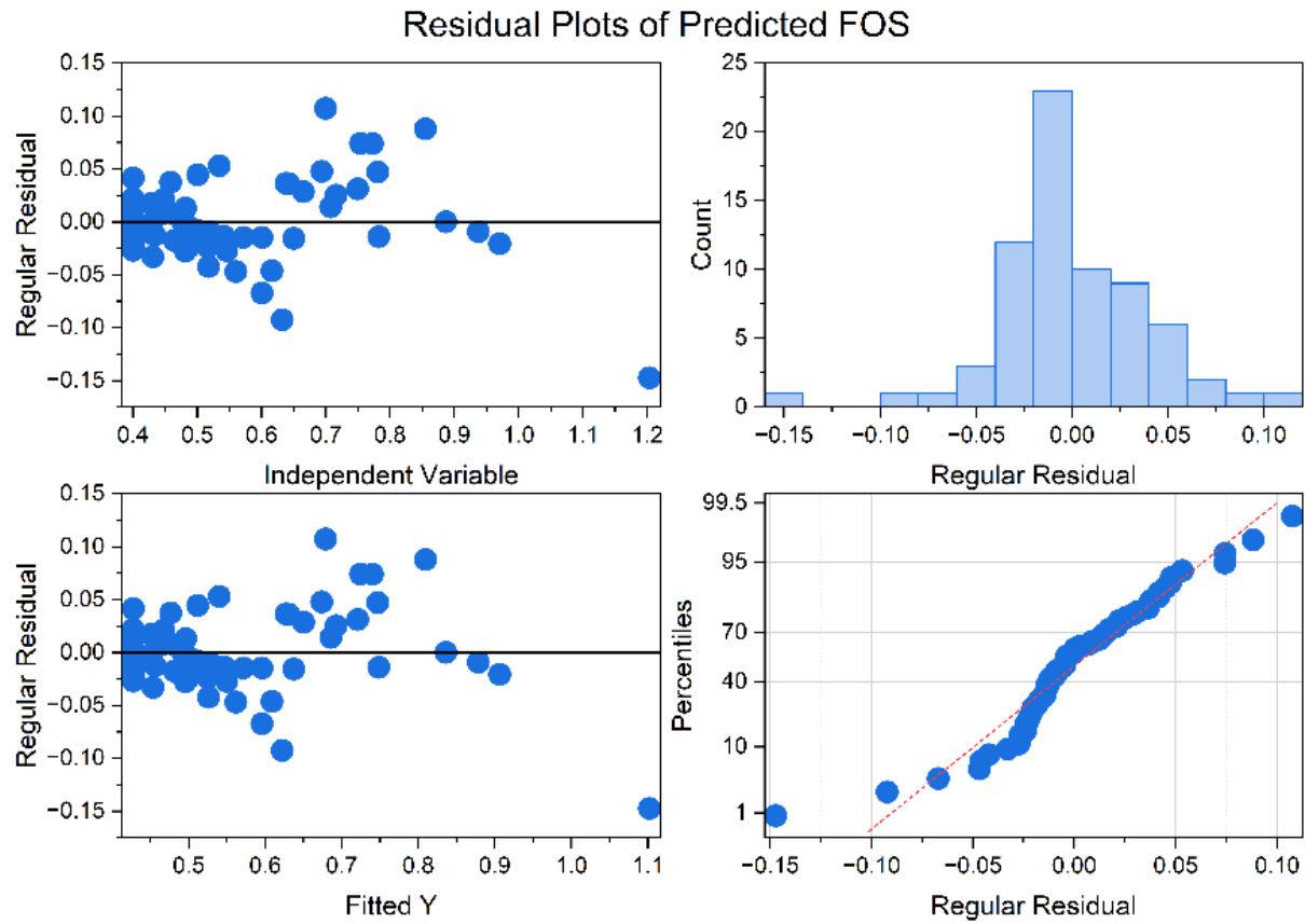
Figure 13. Residual plot for actual vs predicted FoS
