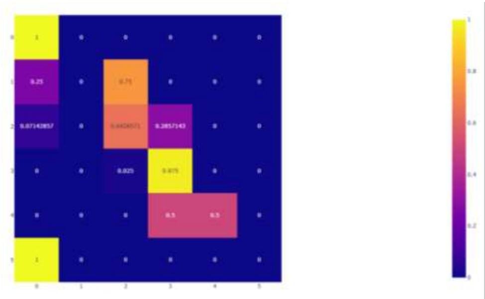
Figure 9. Confusion Matrix for Stability ClassesFigure
