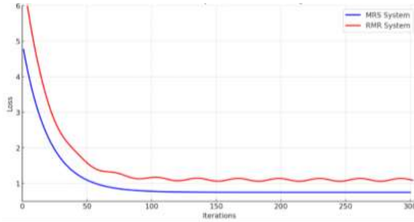
Figure 11. Comparison of ANN training performance between the MRS system and the RMR system.
