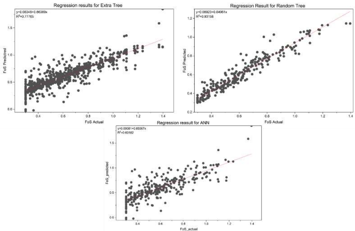
Figure 14. Regression for the validation of fos actual vs fos predicted
