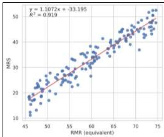
Figure 1. Linear correlation between MRS and RMR indices for the studied deposits.
