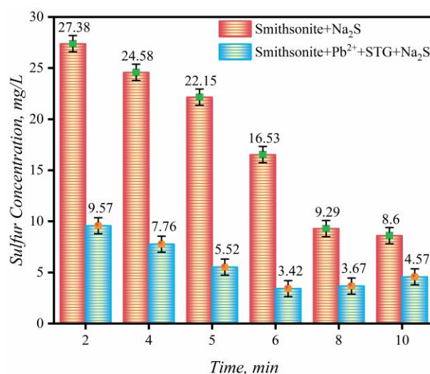
Figure 13. Sulfur concentration in solution as a function of sulfidization time in the presence or absence of \text{Pb}^{2+} and STG.
