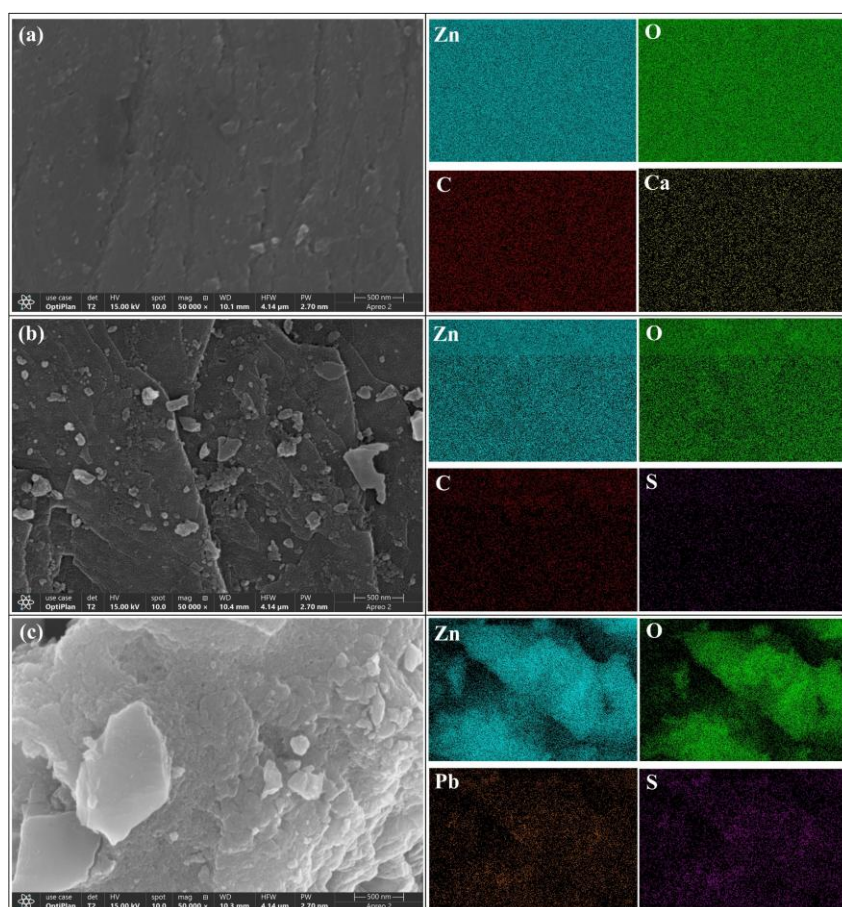
Figure 6. Surface morphologies of pure smithsonite treated with (a) Water, (b) Na 2 S, and (c) Pb 2+ + STG + Na 2 S.
