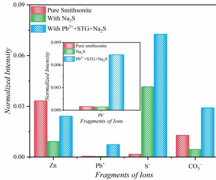
Figure 10. Normalized intensities of ion fragments on the smithsonite surface under the conditions of (a) Water, (b) Na 2 S, and (c) Pb 2+ + STG + Na 2 S.
