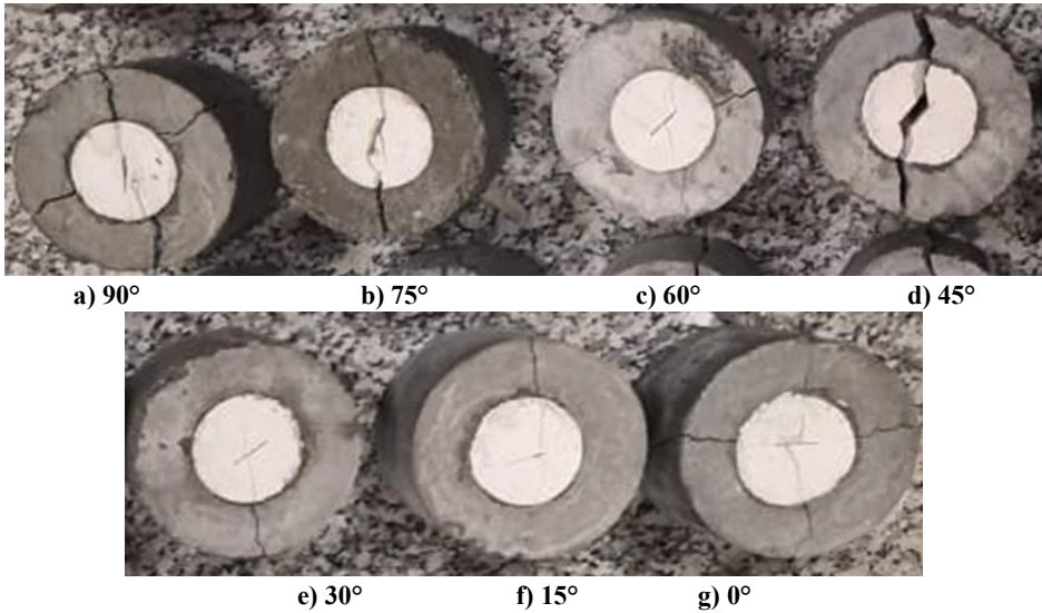
Figure 5. Failure pattern in experimental sample containing the central notch; gypsum diameter was 6cm.
