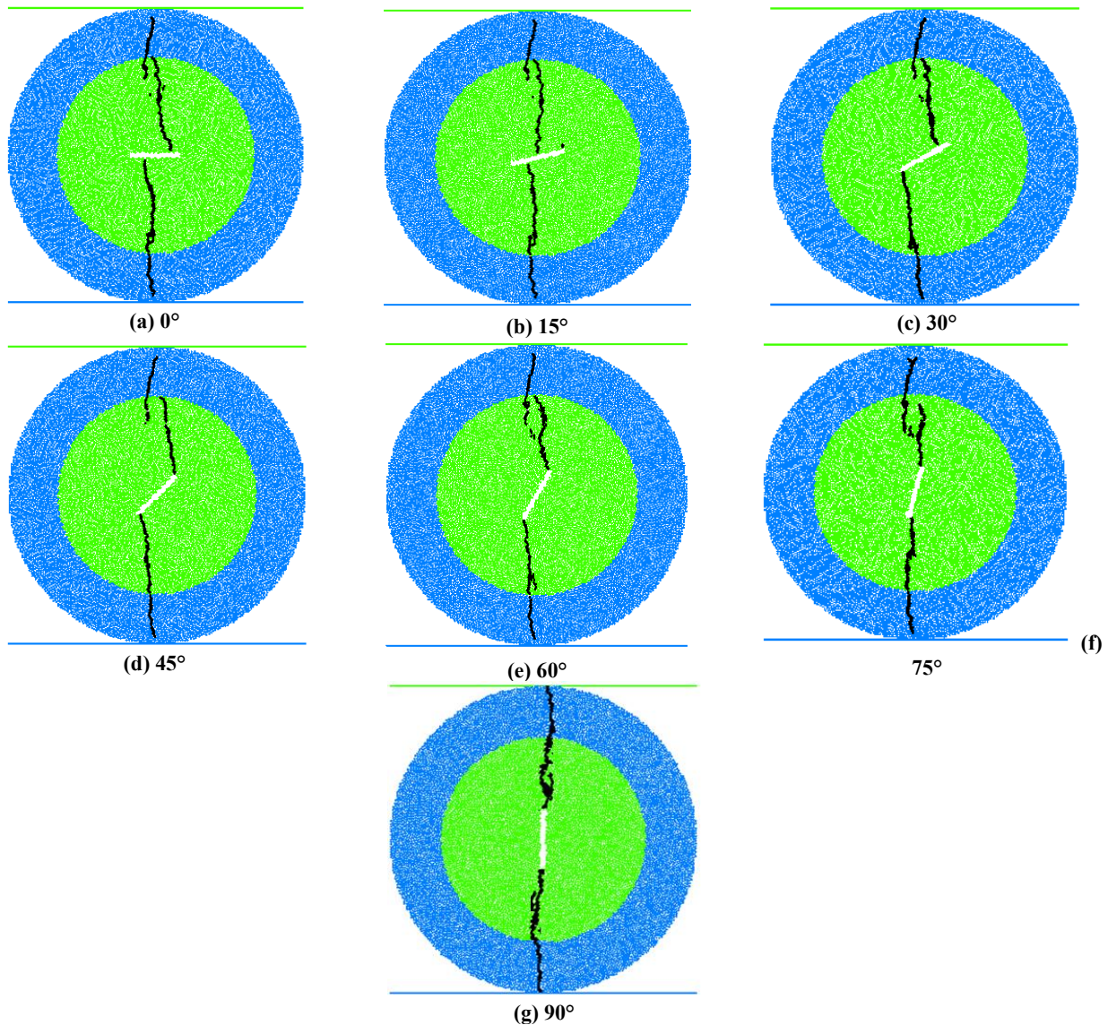
Figure 27: Failure patterns in numerical models with a central notch at various angles, using a gypsum diameter of 9 cm.
