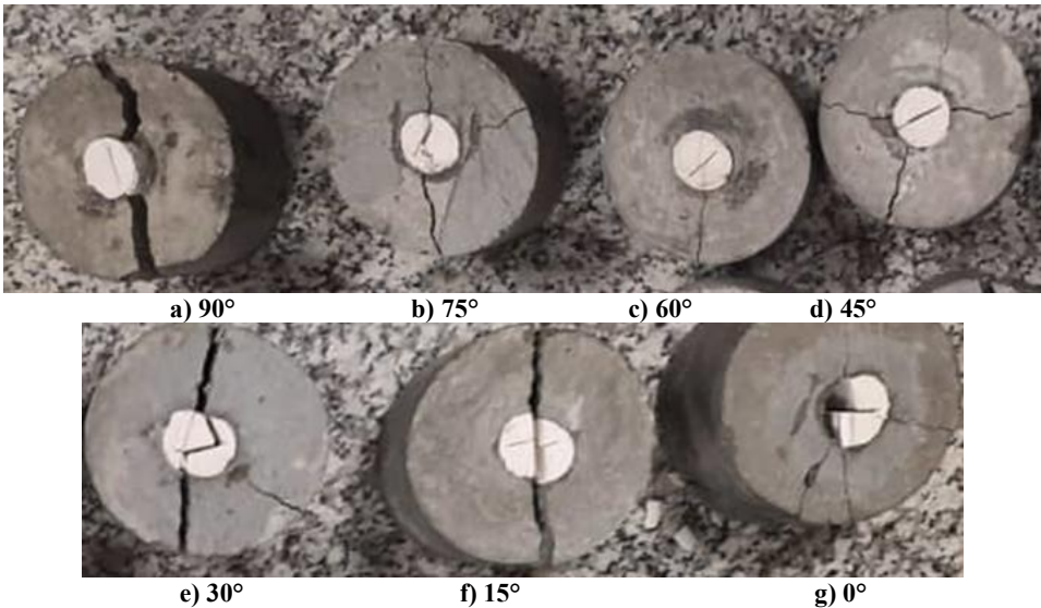
Figure 4. Failure pattern in experimental sample containing the central notch; gypsum diameter was 3cm.
