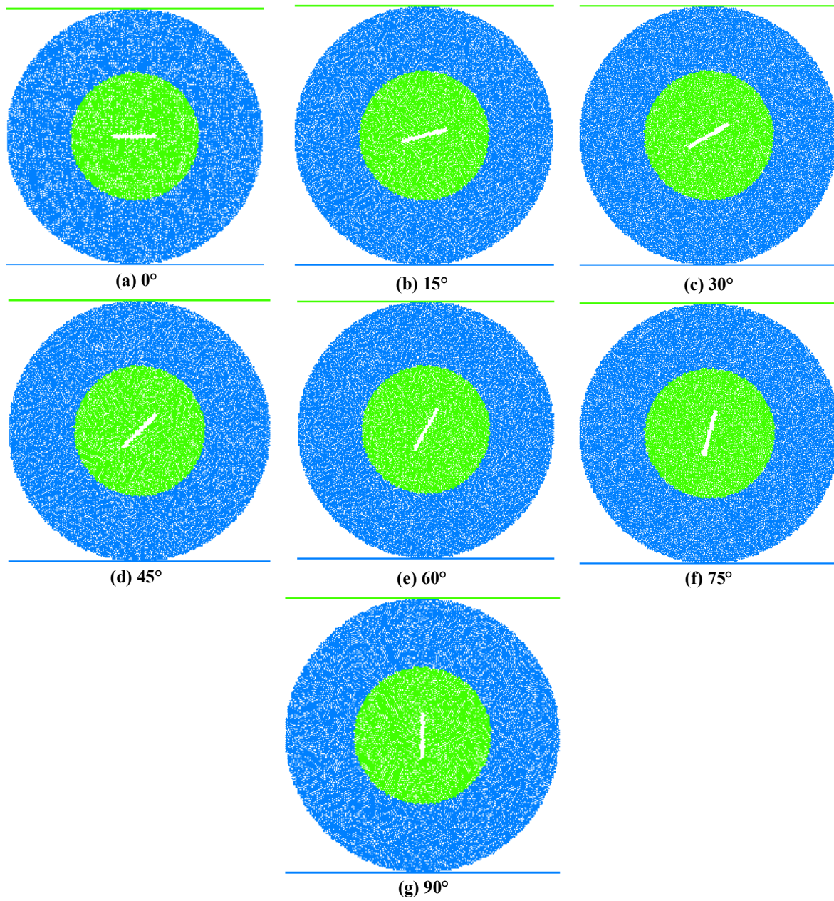
Figure 14. Numerical models featuring a central notch at different angles, with a gypsum diameter of 6 cm.
