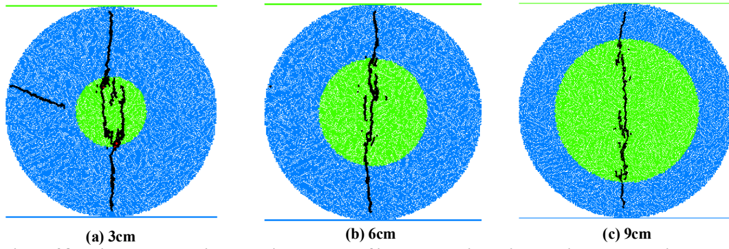
Figure 28. Failure patterns in numerical models of intact materials with varying gypsum diameters.
