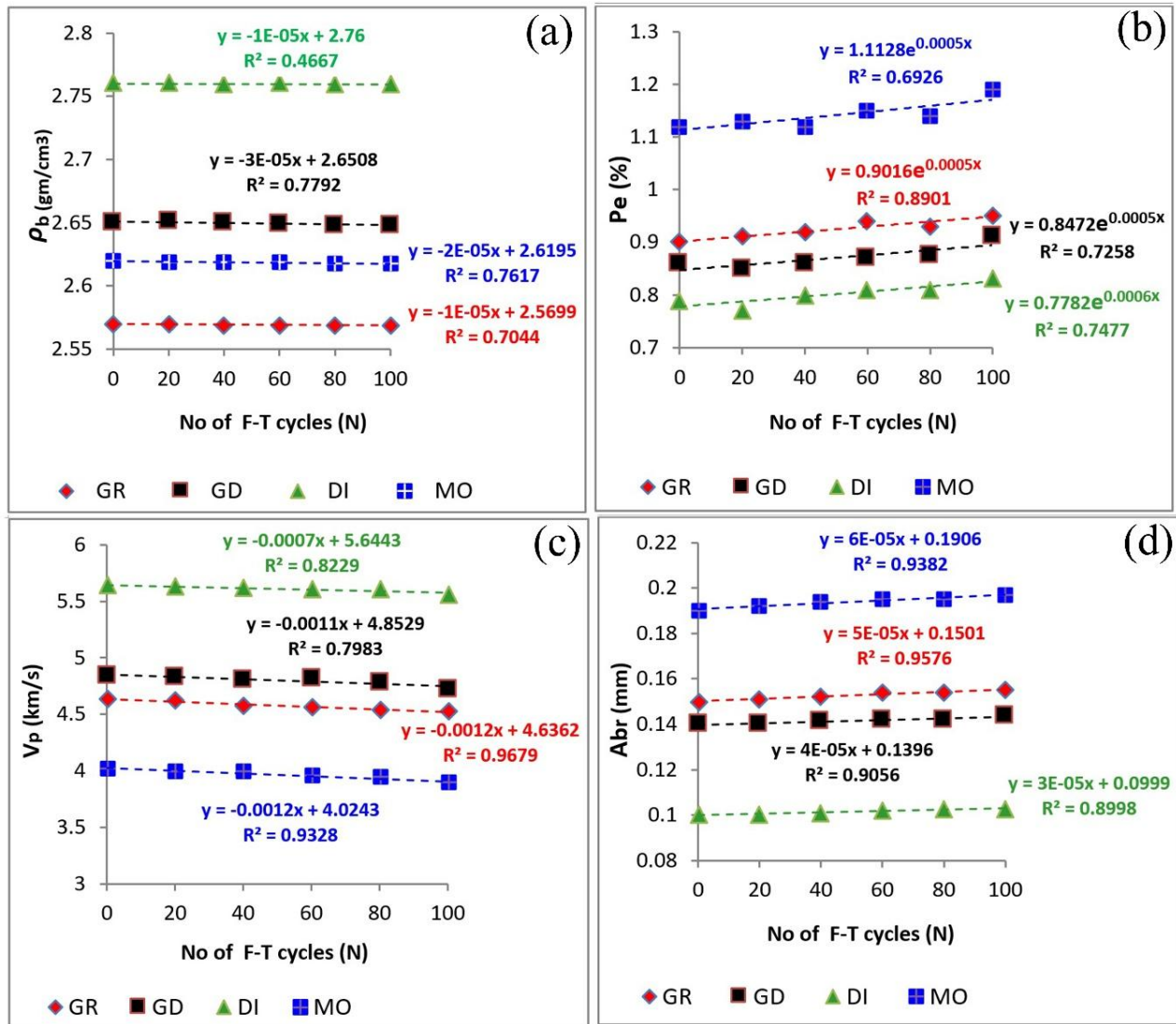
Figure 3. Variations in physico-mechanical properties of the studied igneous rocks under freeze–thaw (F-T) cycles: (a) Dry bulk density ( \rho_b , g/cm 3 ); (b) Porosity ( P_e , %); (c) Ultrasound pulse velocity ( V_p , km/s); (d) Abrasion loss (Abr, mm).
