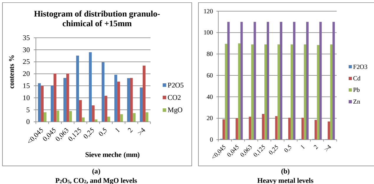
Figure 4. Histogram of P 2 O 5 , CO 2 , MgO and heavy metal Contents (Rejects +15mm)
