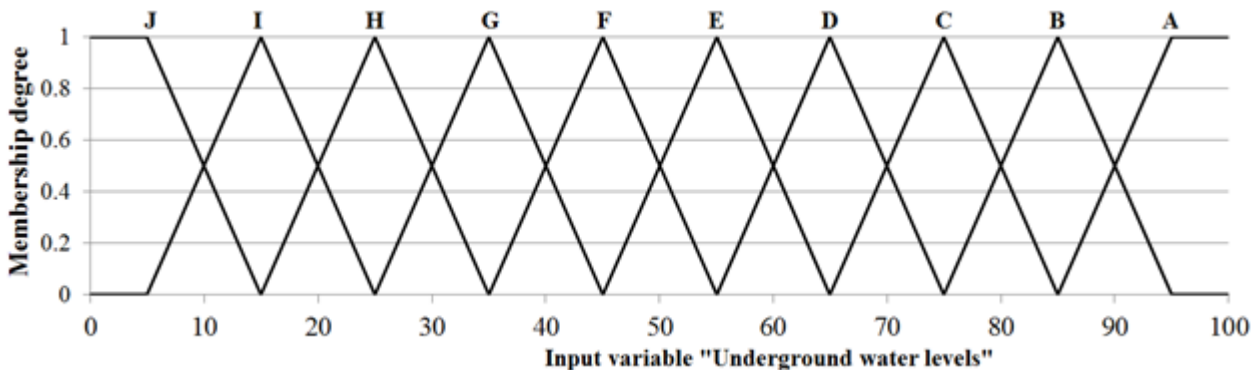
Figure 6. Membership function of input (groundwater levels).
