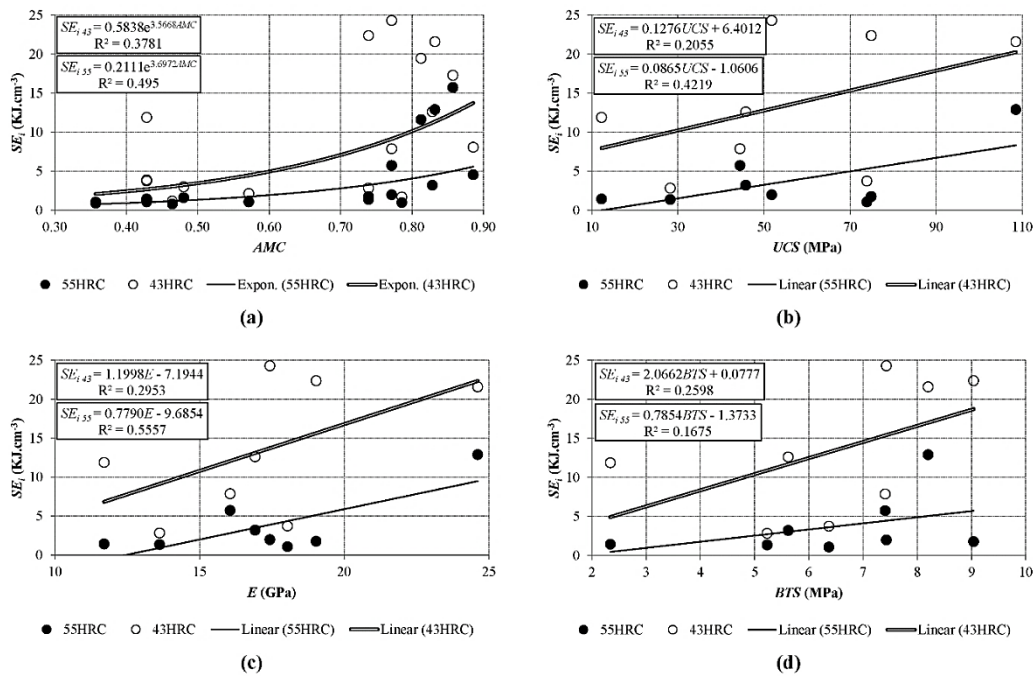
Figure 11. Correlations of scratch energy index ( SE_i ) with a) abrasive mineral contents (AMC), b) uniaxial compressive strength (UCS), c) modulus of elasticity (E), and d) Brazilian tensile strength (BTS) for 43HRC and 55HRC pins.
