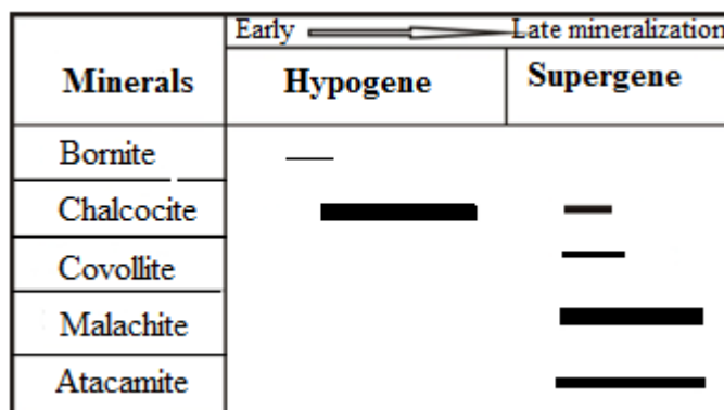
Figure 12. Paragenetic sequence of copper mineralization in studied area.
