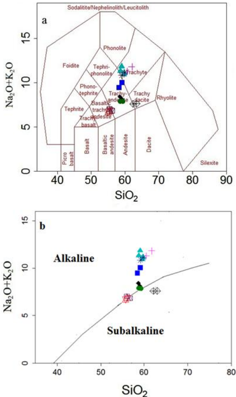
Figure 5. (a) \text{Na}_2\text{O} + \text{K}_2\text{O} vs. \text{SiO}_2 diagram for classification of volcanic rocks [16]; (b) \text{Na}_2\text{O} + \text{K}_2\text{O} vs. \text{SiO}_2 diagram to distinguish between subalkaline and alkaline fields [17].
