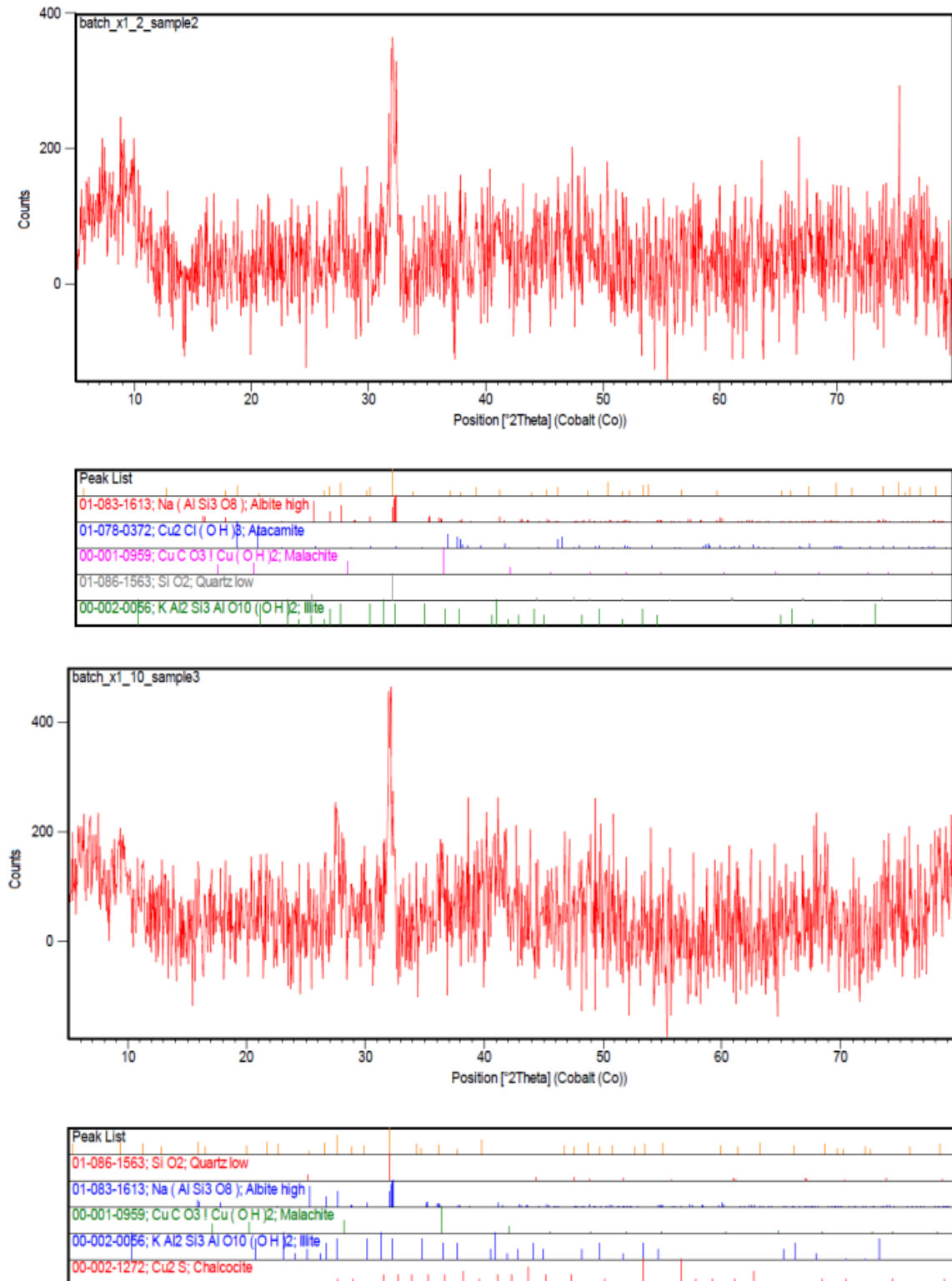
Figure11. Results of XRD test.
