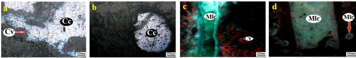
Figure 10. (a) Chalcocite into veinlet is converted to covellite, PPL; (b) Chalcocite into void, PPL; (c) Malachite into veinlet, XPL; (d) Malachite into voids, PPL. (Cc= Chalcocite; Cv= Covellite; Mlc= Malachite).
